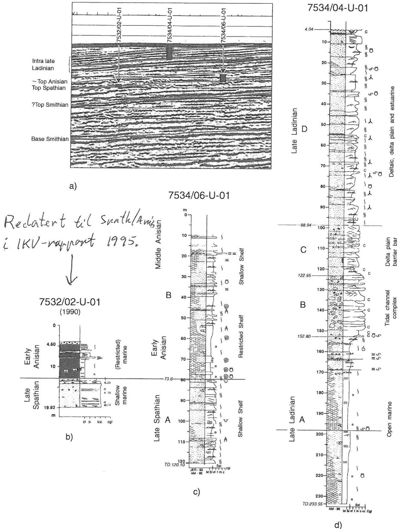
Figure 2.1 a) Seismic line with relative stratigraphic position of the Sentralbanken cores. b) Core 7532/02-U-01 drilled in 1990 which is redated as late Spathian - early Anisian. c) Core 7534/06-U-01 of late Spathian to Middle Anisian age. d) Core 7534/04-U-01 of late Ladinian age.
