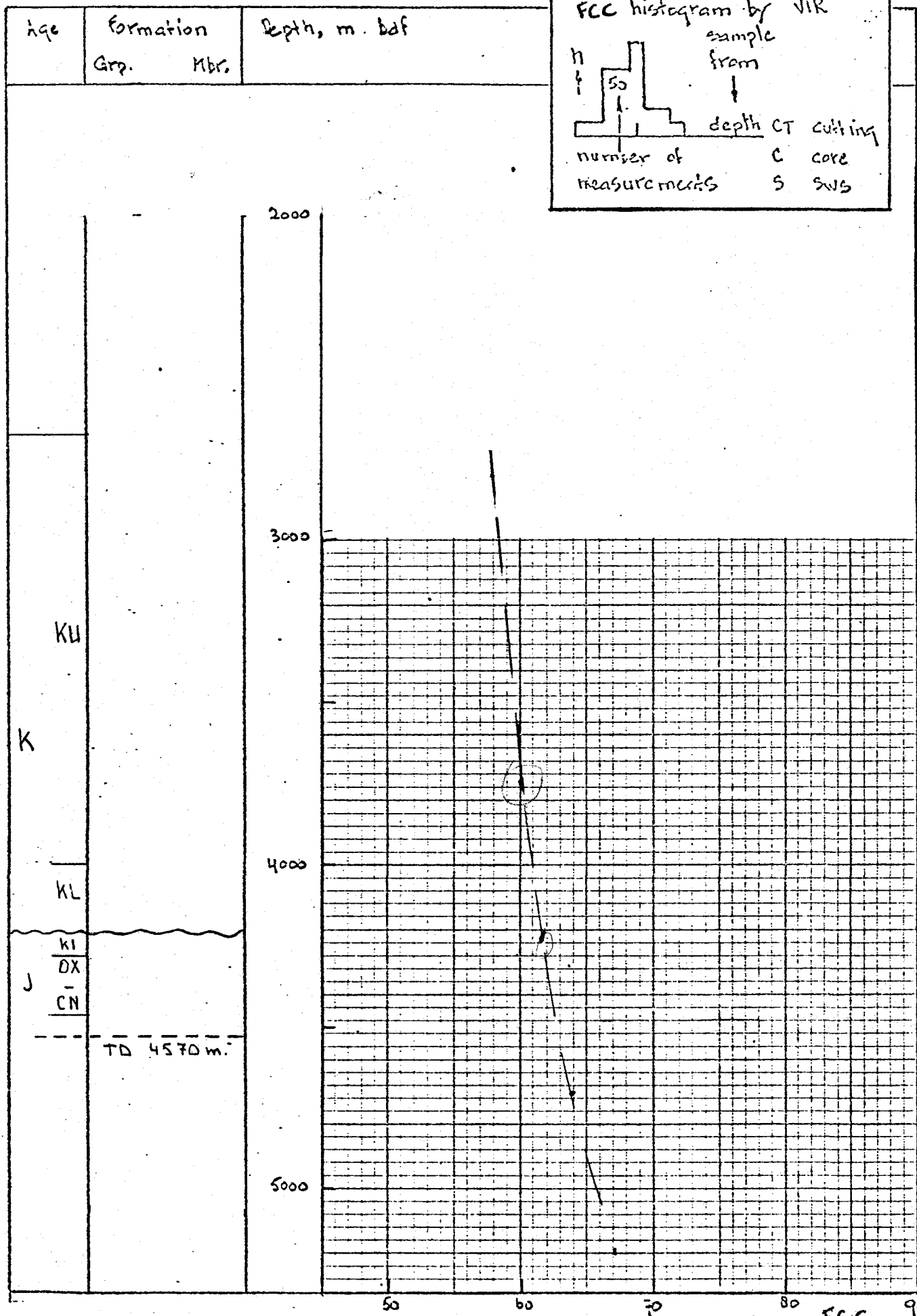
FCC AS A FUNCTION OF DEPTH, WELL 25 | 1 - 1
