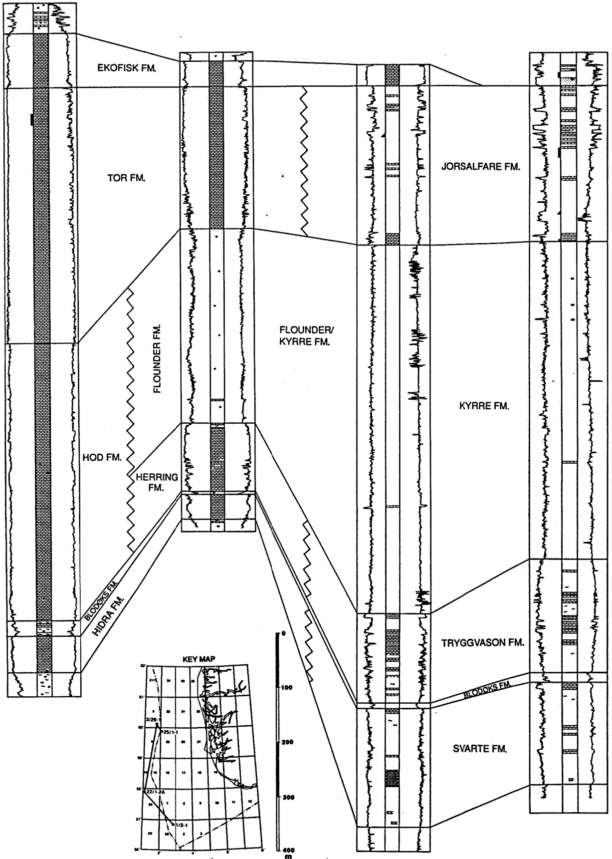
Well correlation in the Central trough and the Viking Graben
