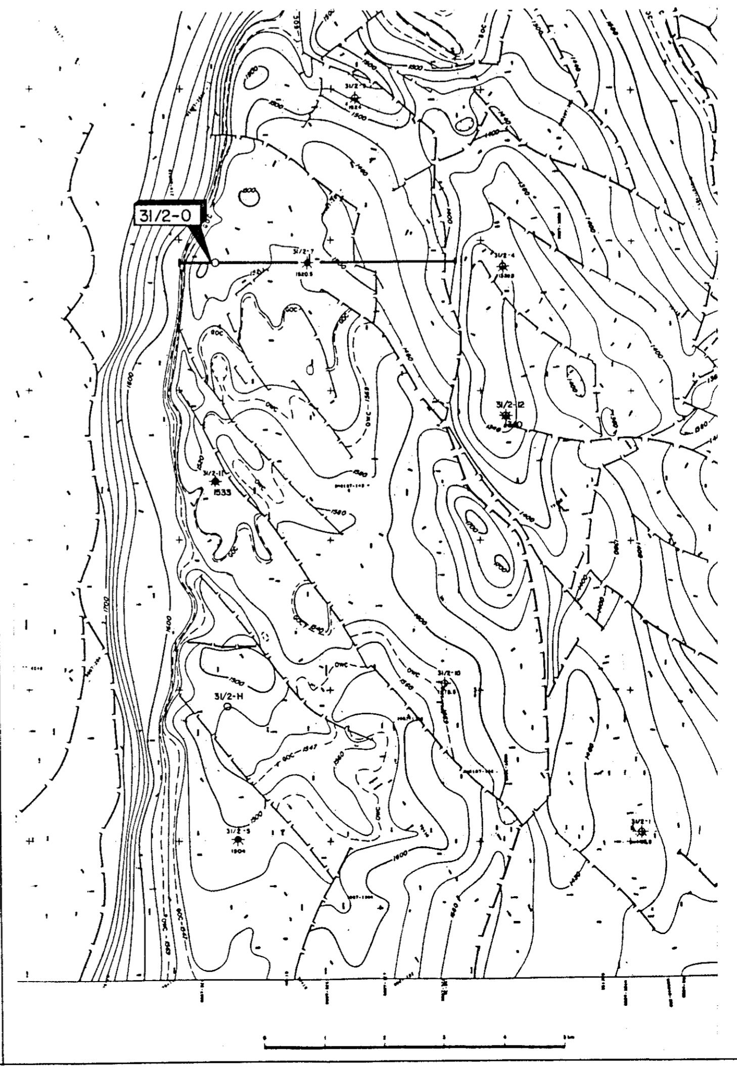
LOCATION OF APPRAISAL WELL 31/2 - 0 SHOWN ON TOP RESERVOIR
