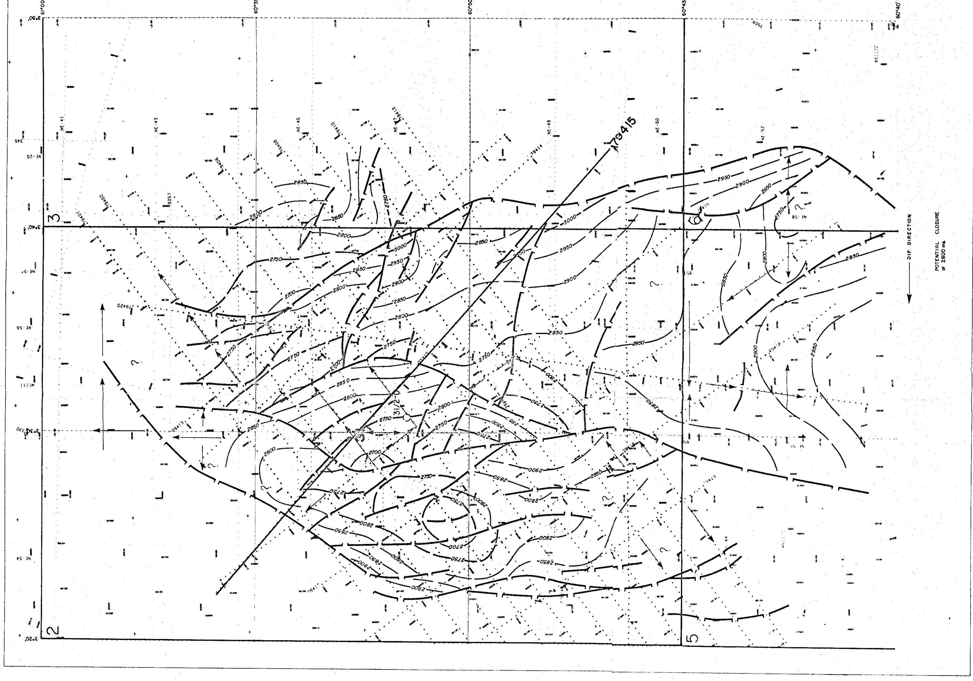
LOCATION MAP 1:100000
