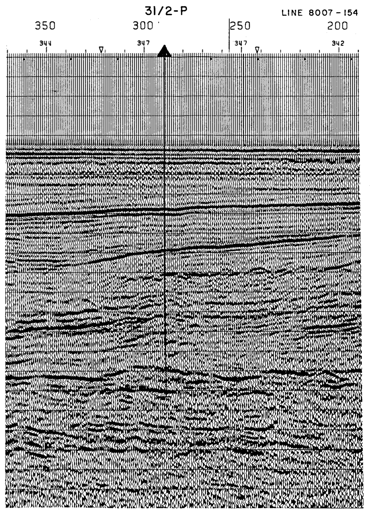
LOCATION OF APPRAISAL WELL 31/2-P SHOWN ON TOP RESERVOIR
