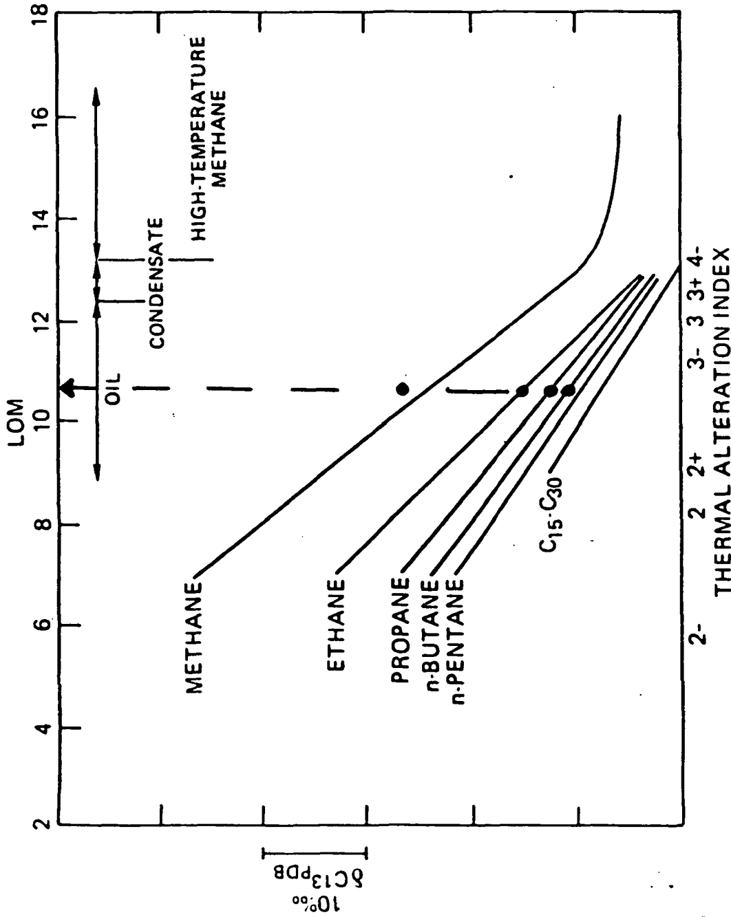
Figure 1. Carbon isotopic separations of the gas from well 30/2-11 is plotted on the maturity diagram (after James, 1983). A source LOM between 10 and 11 is indicated for the gas.
